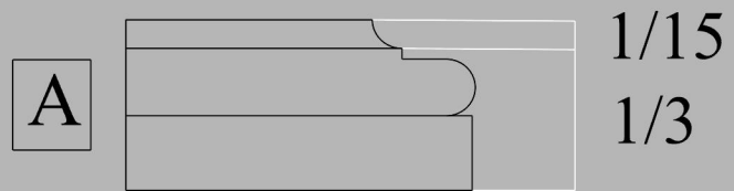
Base tuscanica Ledoux
